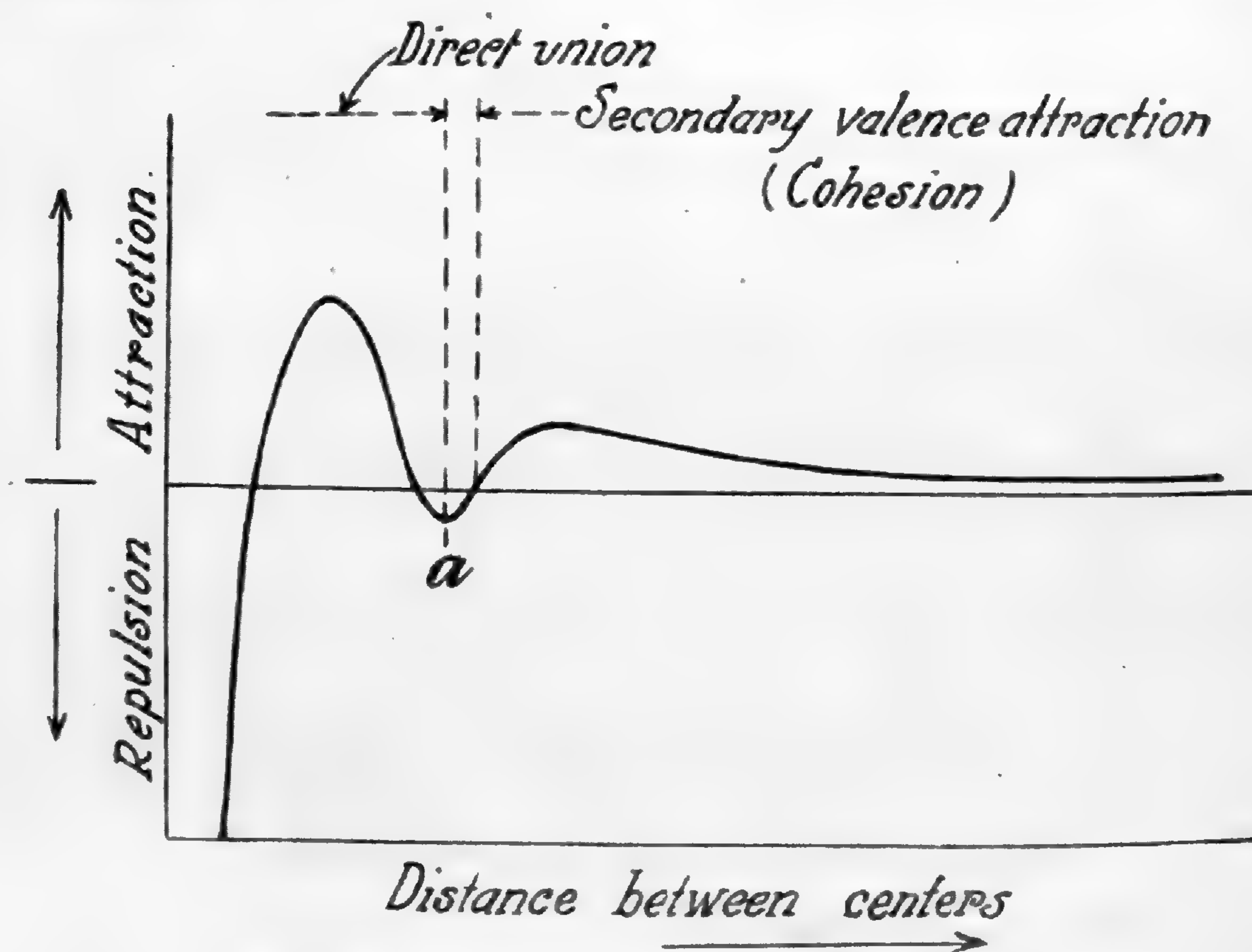
FIG. 6. The attraction between two reacting molecules.
